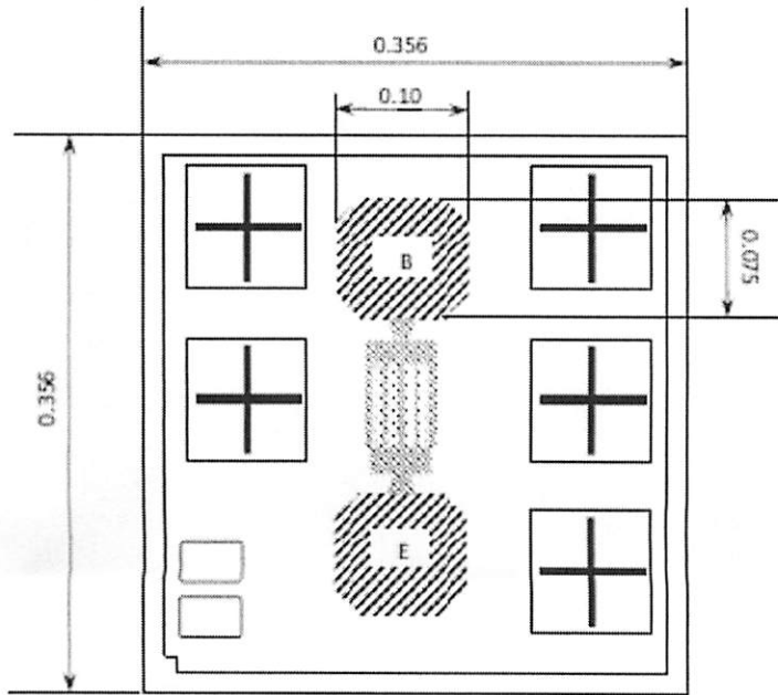
Chip Back Is Collector
